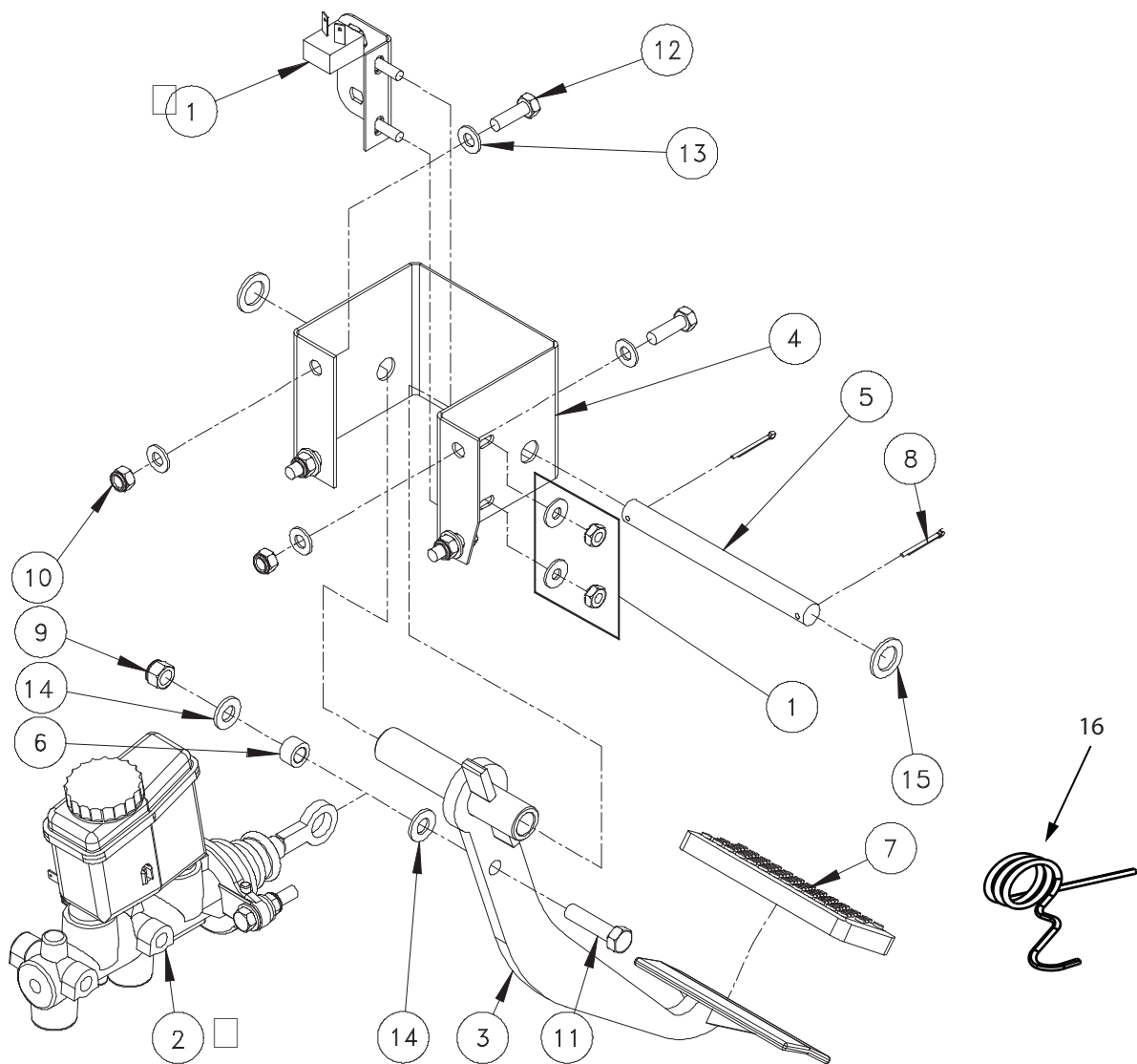
ASSY,BRAKE PEDAL06
