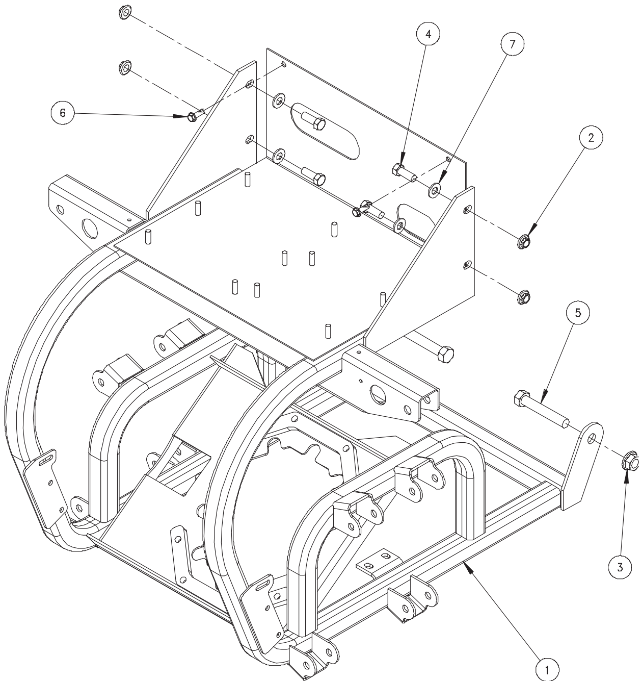
ASSY,SUPPORT FRAME - FRONT 46 IN WIDE
