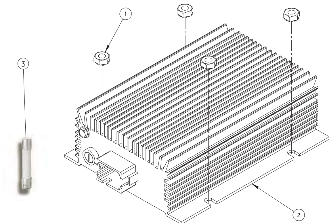
ASSY, CONVERTER - 72 V/12V 30 AMP (SURE POWER)
